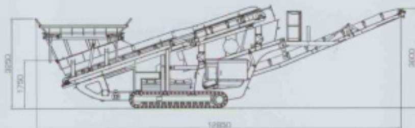
Working position
