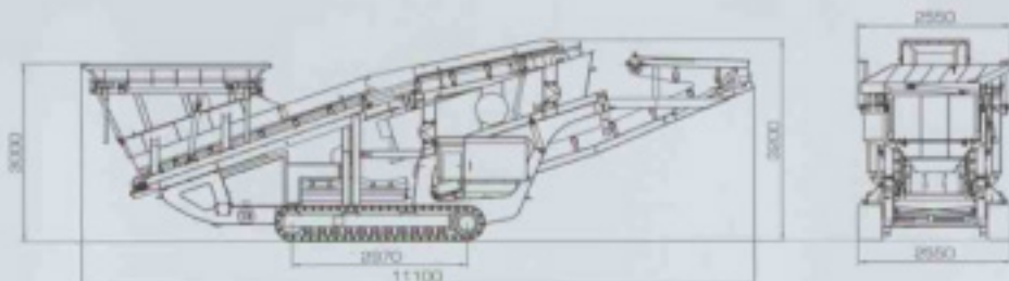
Transport position
